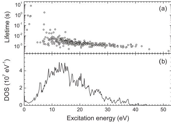
FIG. 3. (a) Calculated excitation energies and lifetimes of 292 out of all 293 excited fine structure components of the W^{20+}([Kr]4d^{10}4f^8) ground configuration. The calculated lifetime of the {}^3O_{12} state is off scale. (b) Calculated density of states (DOS) comprising all doubly excited 4f^8 nl states above the W^{20+}(4f^8 {}^7F_6) ground state with n \leq 72 .
