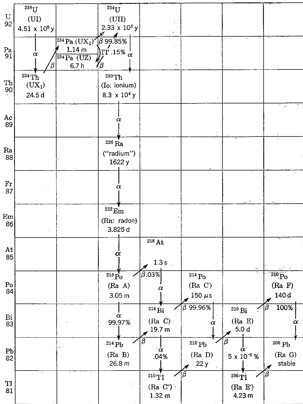
FIG. 15-3. The uranium (4n + 2) radioactive series.
