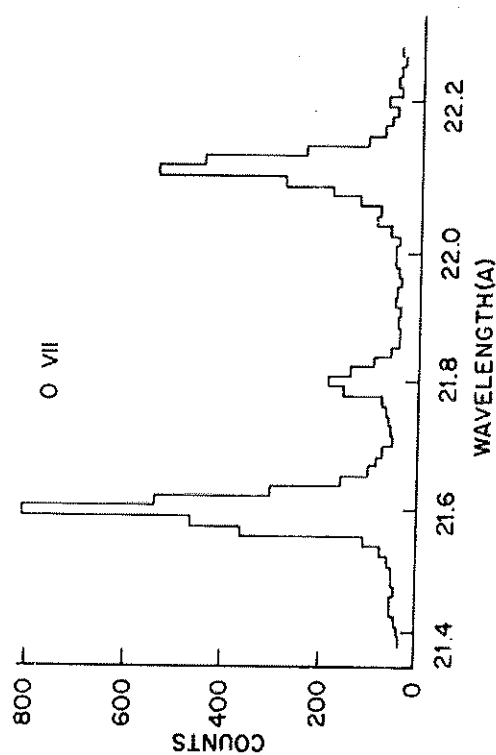
Fig. 3. O VII and Ne IX spectra of McMath plage No. 281 accumulated during flight in approximately five seconds. Resonance, intersystem and forbidden transitions are labelled R, I and F respectively.
