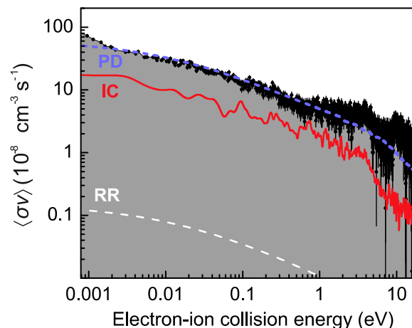
Figure 11. Dielectronic recombination cross-section of W^{18+} ions ( 4f^{10} valence configuration) measured with the storage-ring merged-beams method. (Cross section \sigma multiplied with the collision velocity v and convolved with the electron energy spread.) Calculations show radiative recombination (RR), dielectronic recombination by one-electron promotion in intermediate coupling (IC), and a model including statistical partitioning and a damping correction (PD). (Adapted from [72], copyright 2014 by the American Physical Society. Beam-merging artefacts at < 0.001 \text{ eV} are negligible in the plasma rate constants.)
